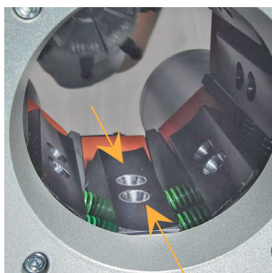
With the double pin connection, it is possible to crimp on both sides of S3 series machines.
