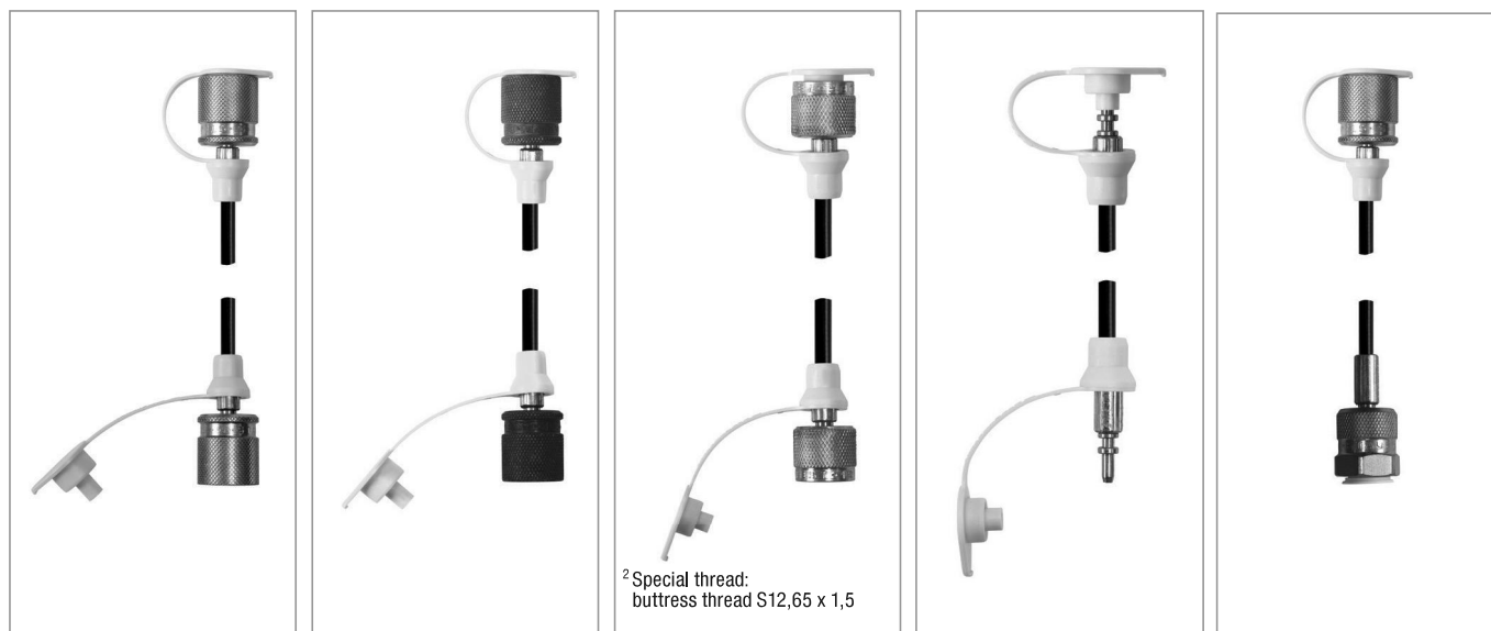
STAUFF-Test 12/12 2
